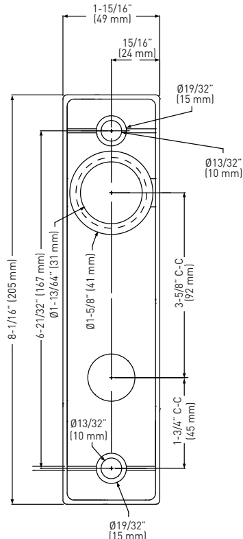
ESCUTCHEON PLATE EXTERIOR
