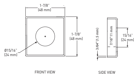
SQUARE SECTIONAL ROSE: LEVERS
