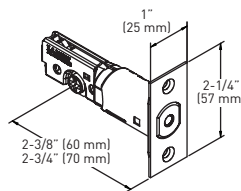
2-IN-1 DEADBOLT LATCH
