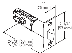
2-IN-1 SPRING LATCH
