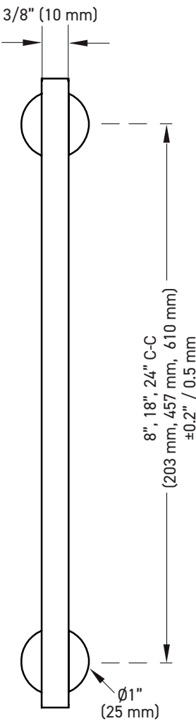
FRONT ELEVATION
