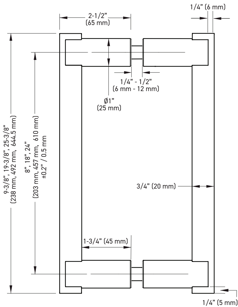
SIDE ELEVATION
