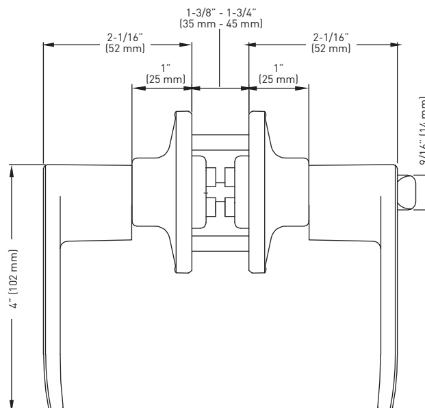
4-IN-1 DRIVE-IN/SQUARE MORTISE
