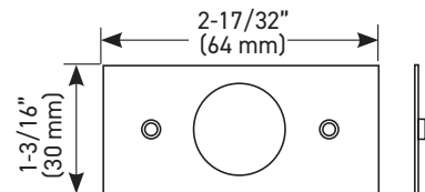
EXTERIOR BRACKET
